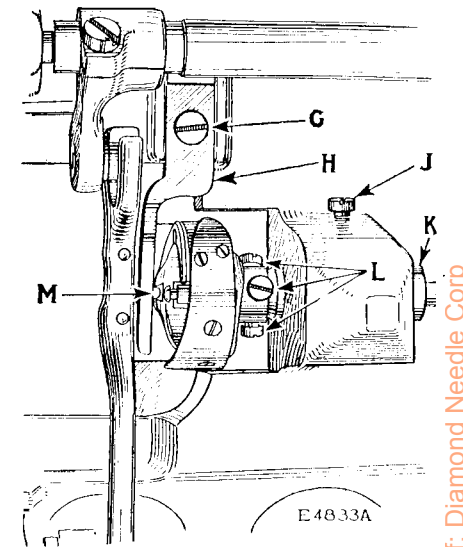
FIG. 20. VIEW OF UNDERSIDE OF MACHINE SHOWING BOBBIN CASE HOLDER POSITION BRACKET (H) AND ADJUSTMENTS ON MACHINE
